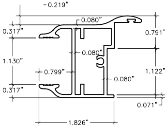
3 SASH PERIMETER
