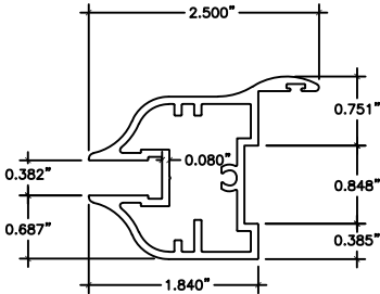
*3B SASH PERIMETER 5/16" GLASS
